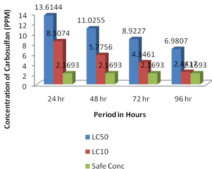
Figure-2. Comparison of LC50, LC10 and safe concentration at different exposure periods of Carbosulfan
