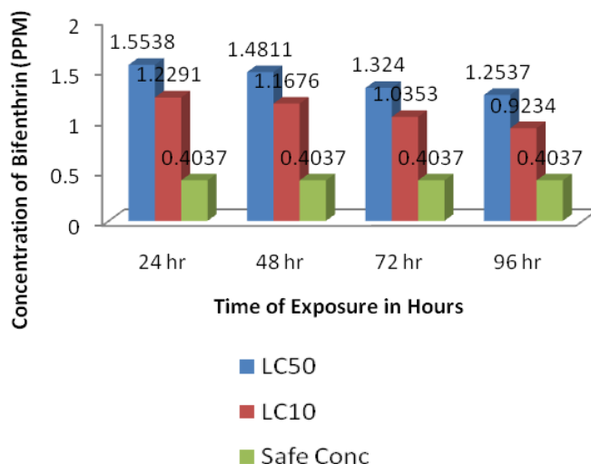
Figure-1. Comparison of LC10, LC50 and safe concentration at different exposure periods of Bifenthrin
