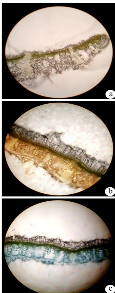
Figure-2. Leaf anatomy (100x) of Pistia stratiotes Engl. Showing bioaccumulation of chromium and copper. a) Control; b) Bioaccumulation of chromium in mesophyll tissue; c) Bioaccumulation of copper in mesophyll tissue.
