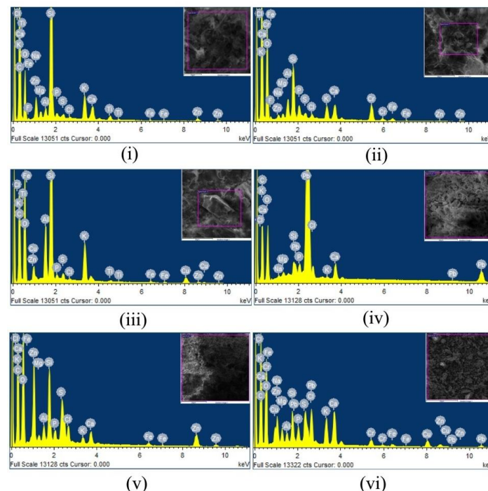
Figure-3. Elemental analysis of Pistia stratiotes Engl. Using SEM-EDX. i) Control; ii) Bioaccumulation of chromium; iii) Copper; iv) Lead; v) Zinc; vi) Bioaccumulation of metals and its product after combustion
