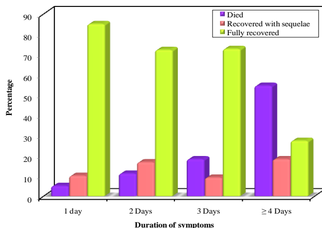
Figure-5. Relation between outcome and duration of symptoms
