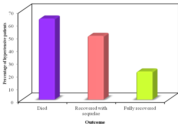
Figure-7. Relation between outcome and chronic hypertension
