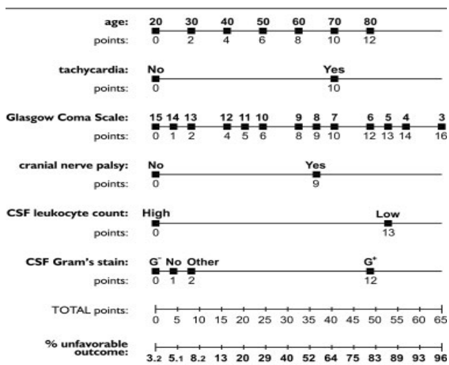
Figure-9. Weisfelt's Bedside risk score for adverse outcome within the first hour after admission in adults with acute bacterial meningitis.
