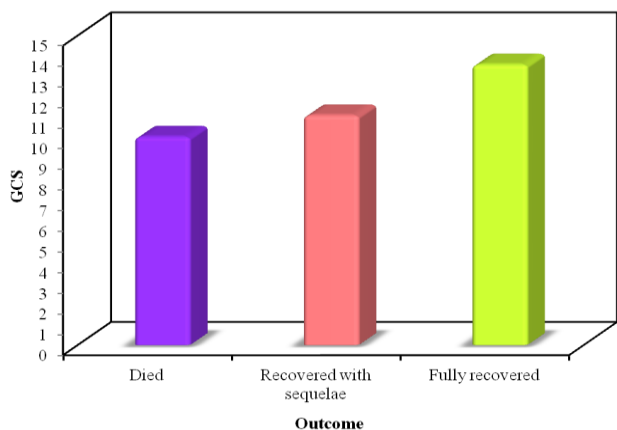
Figure-4. Relation between outcome and Glasgow coma score (GCS).
