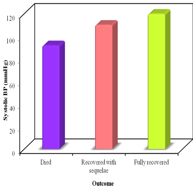
Figure-3. Relation between outcome and Systolic blood pressure (mmHg)
