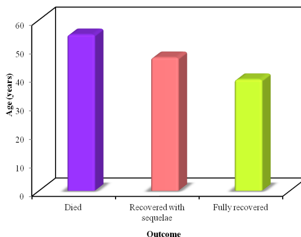
Figure-2. Relation between patients' age and outcome.
