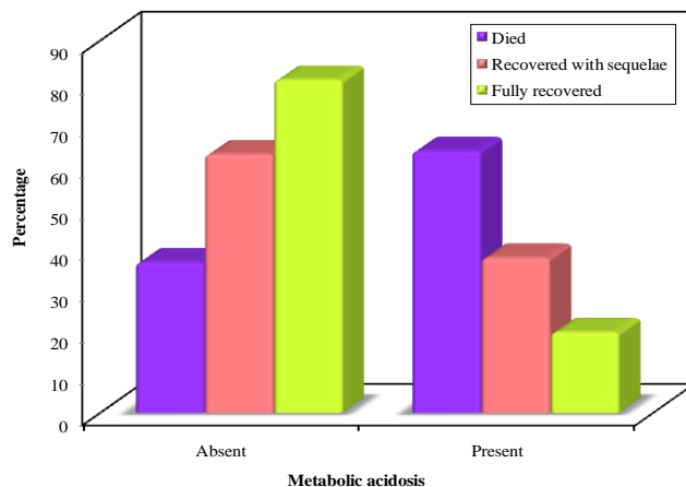
Figure-6. Relation between outcome and metabolic acidosis
