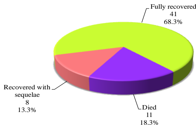
Figure-1. Classification of the patients according to the outcome.
