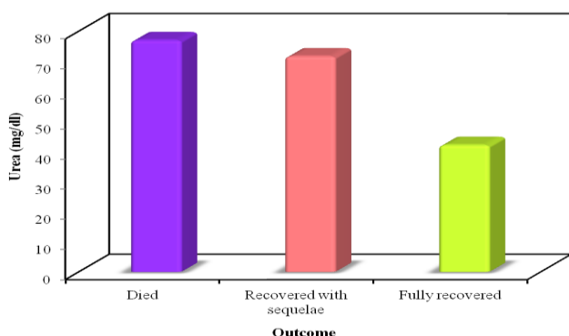
Figure-8. Relation between serum urea and outcome.
